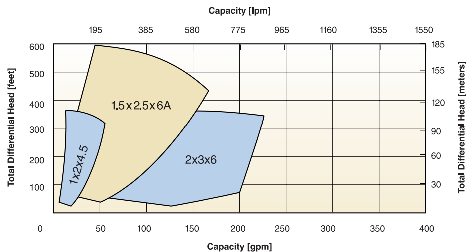
AC-18HD Boost Pump
