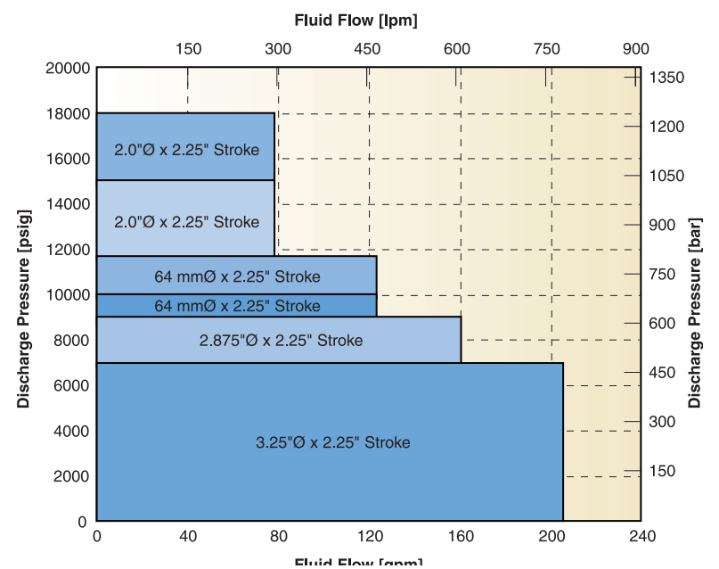
3-SLS 1100 Horsepower Cryogenic Reciprocating Pump
