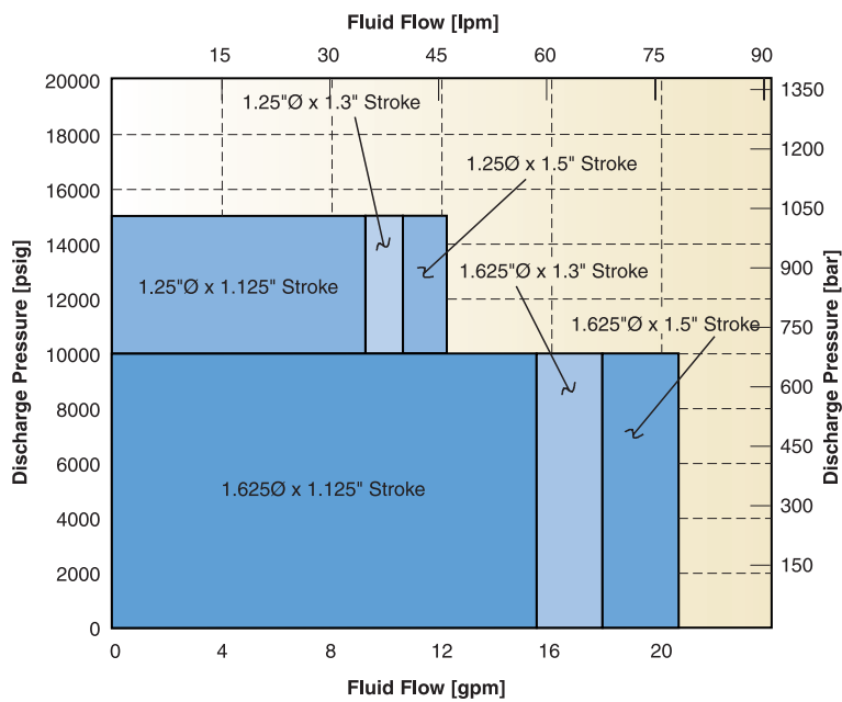
3-SZGU Cryogenic Reciprocating Pump
