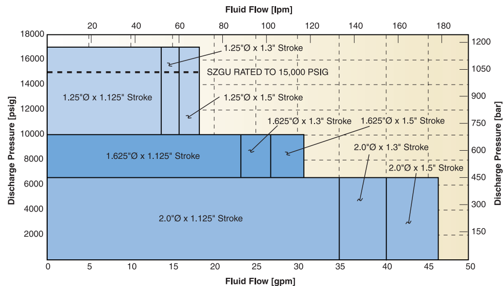
3-GUPD Cryogenic Reciprocating Pump
