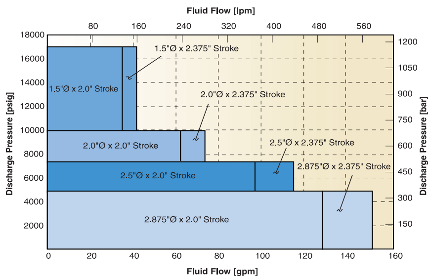
3-LMPD Cryogenic Reciprocating Pump
