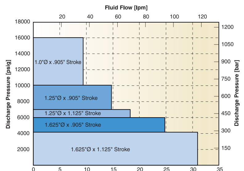
3-GMPD Cryogenic Reciprocating Pump
